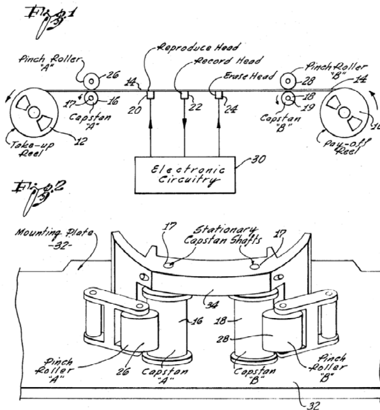
Patented Tape Drive System
