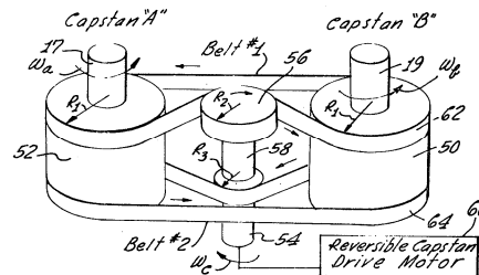
Bi-Directional Capstan Drive Patent (No Pinch Rollers)
